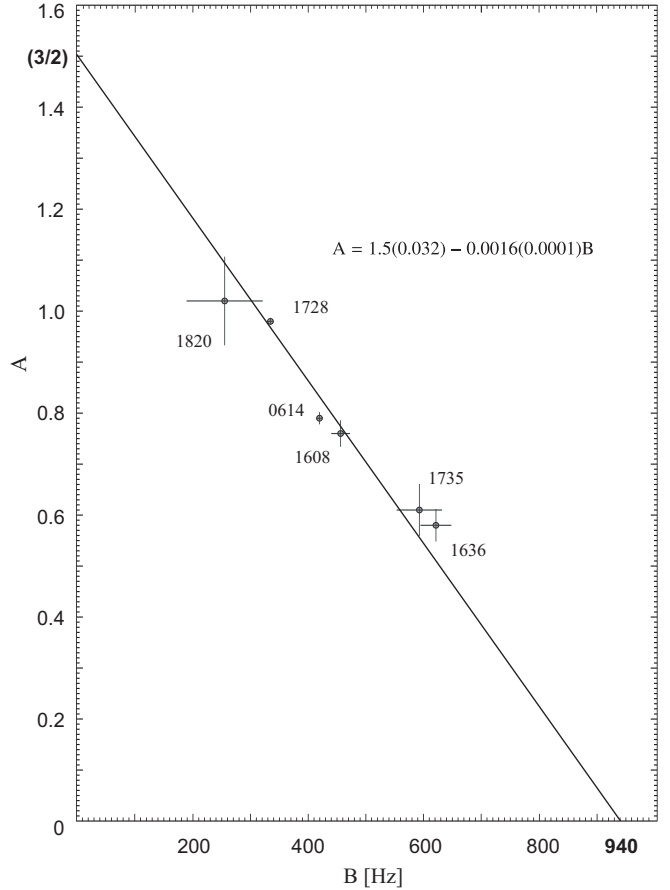
Fig. 1. The anticorrelation between the shift and slope. The figure shows the result obtained from the analysis of the data. Each point in the plot corresponds to the particular source. The shift A and the slope B correspond to the best linear fit of the \nu_1 - \nu_2 correlation. Clearly, A and B are anticorrelated among the sources. The linear fit for the anticorrelation and the errors of the fit are given in the figure. Note that value of the fit crosses vertical axis very close 1:5. This fact is in agreement with the idea that the excitation mechanism of QPOs is 3:2 resonance.
