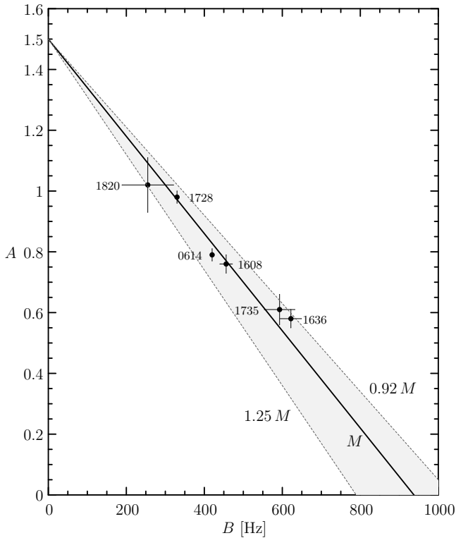
Fig. 2. The effect of 1/M -scaling on the anticorrelation between the shift and slope. The solid line is the best fit of the anticorrelation given by equation (3). In the spirit of 1/M , it corresponds to a ‘typical’ neutron-star mass between the examined system. Dashed lines represent the best fit rescaled to 0.92M and 1.25M . The
