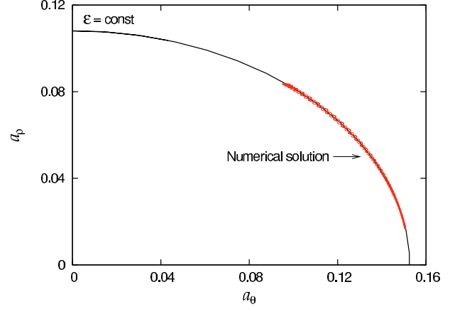
Fig. 3. Comparison between the analytical constraint \mathcal{E}(a_\rho, a_\theta) = \text{const.} (an ellipse), derived in a multiple-scales approximation, and the corresponding exact (numerical) solution. The curly curve is the numerical solution of the oscillation amplitudes a_\rho(t) , a_\theta(t) . The agreement between the two curves demonstrates that the accuracy of the approximation is satisfactory over the entire time span. See the text for details.
